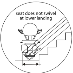
Lower Landing 18"-20" Normal Rail Extension
